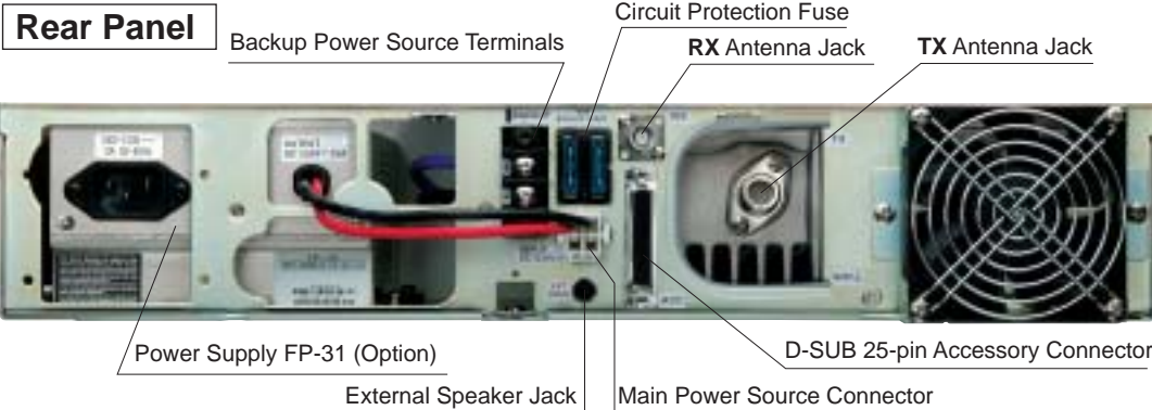
VPA-9000 V-H / U-H (VHF) (UHF) 100 W Power Amplifier Unit
